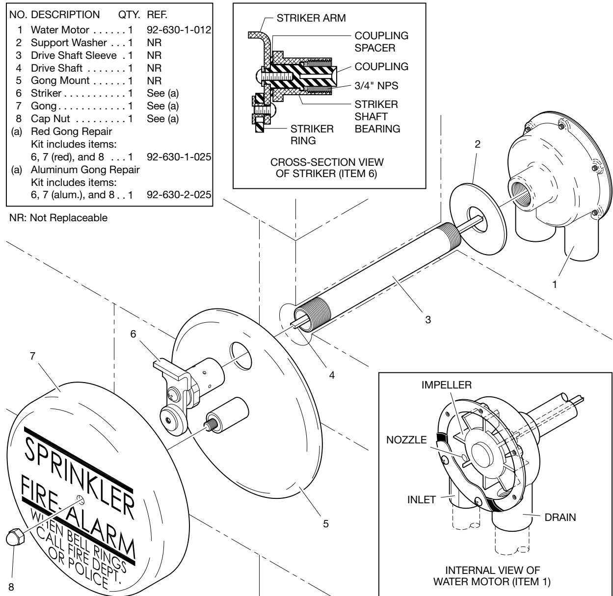
FIGURE 1 MODEL WMA-1 WATER MOTOR ALARM ASSEMBLY
