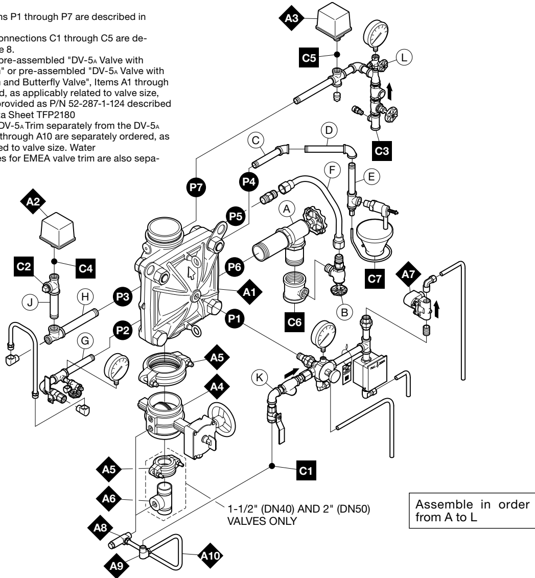
FIGURE 5 DV-5A VALVES DOUBLE INTERLOCK PREACTION ELECTRIC/ELECTRIC ACTUATION TRIM SEMI-ASSEMBLED
