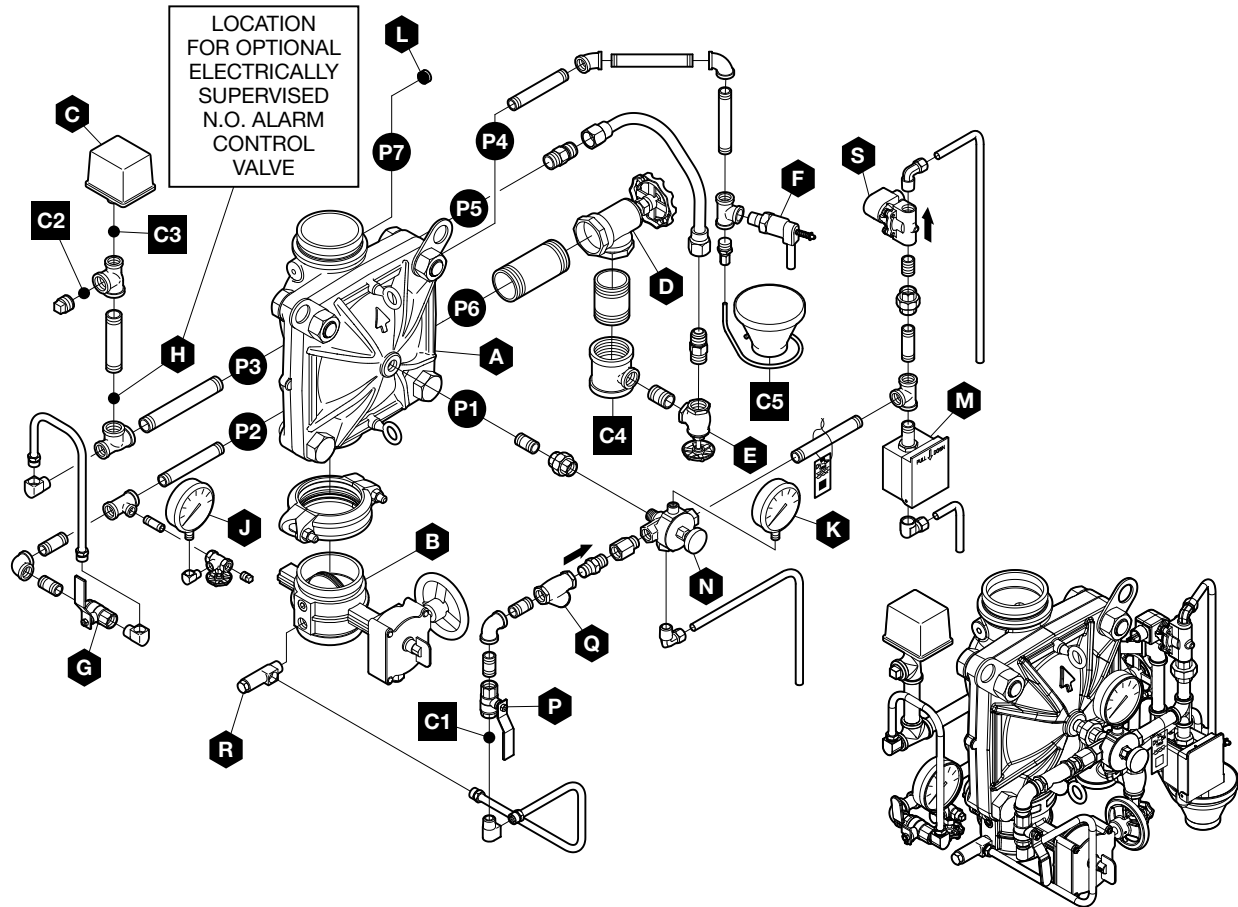
FIGURE 8 DELUGE ELECTRIC ACTUATION TRIM (REFER TO FIGURE 6 FOR SPECIFIC BILLS OF MATERIALS)
