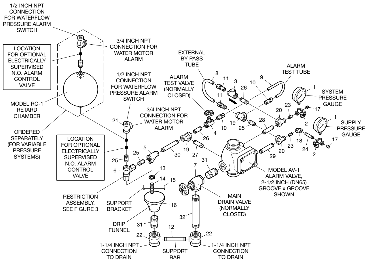
FIGURE 5 (1 OF 3) VERTICAL OPEN DRAIN TRIM – SPECIAL ORDER FOR 2-1/2 INCH (DN65) MODEL AV-1-300 ALARM CHECK VALVES (P/N 52-204-4-953)
