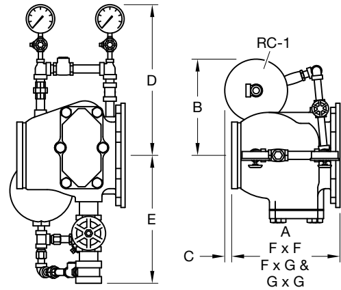
FIGURE 7 (3 OF 3) INSTALLATION DIMENSIONS FOR 8 INCH (DN200) MODEL AV-1-300 ALARM CHECK VALVES
